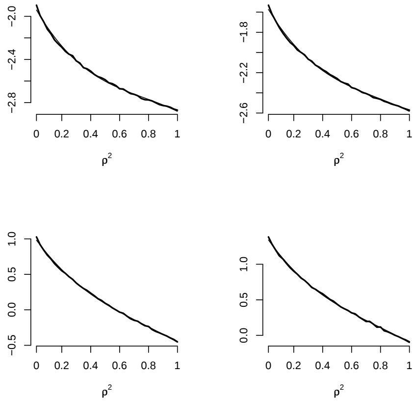
Figure 2: Interpolation of the quantiles \widehat{q_\rho(p)} . From upper-left clockwise: \alpha = 5\% , \alpha = 10\% , \alpha = 95\% , \alpha = 90\% . The thick solid lines are the simulated quantiles. The thin lines are the interpolated values.
