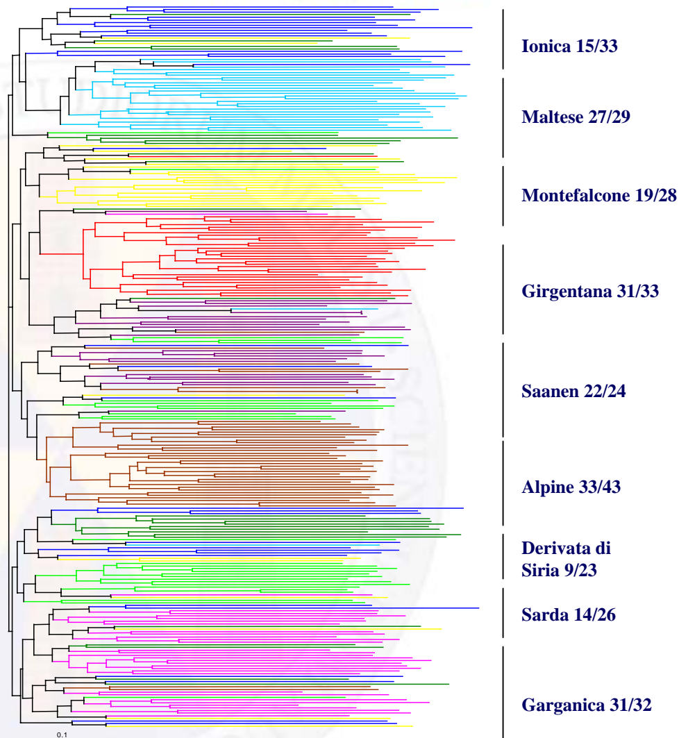
Neighbour-Joining diagram of distances among individuals
